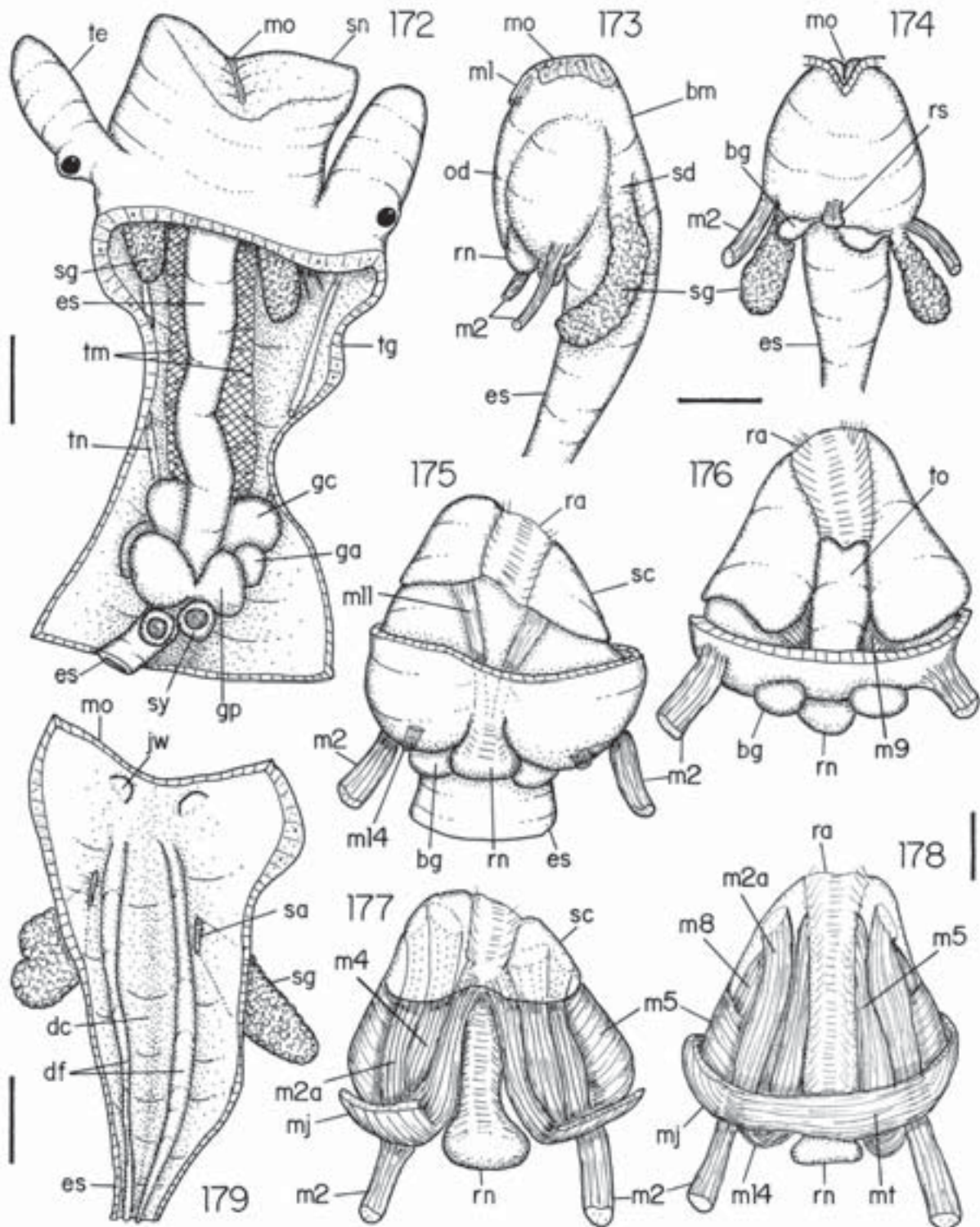
Figures 172-179, Calyptraea centralis anatomy: 172 , head and haemocoel, ventral view, foot and neck ventral surface extracted; 173 , buccal mass and adjacent esophagus, lateral-left view; 174 , same, dorsal view; 175 , odontophore, ventral view; 176 , same, dorsal view; 177 , odontophore, ventral view, superficial membrane and muscles removed; 178 , same, dorsal view; 179 , dorsal wall of buccal mass, ventral view, odontophore and septum between it and esophagus extracted, esophagus also opened longitudinally. Scales 172, 179 = 0.25 mm; 173-178 = 0.1 mm.
